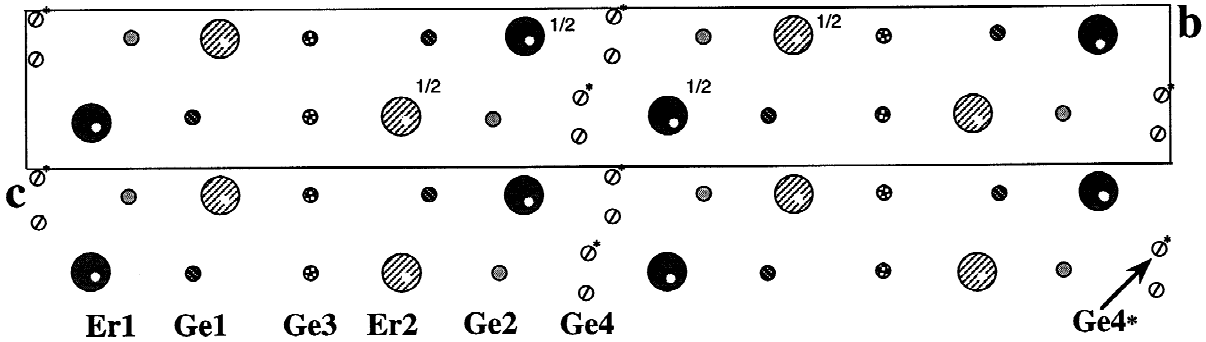
Fig. 4. The unit cell projection of \text{ErGe}_{1.83} structure at (0,y,z) plane. In the Cmcm space group germanium atoms occupy positions marked as Ge4 and \text{Ge4}^* .
