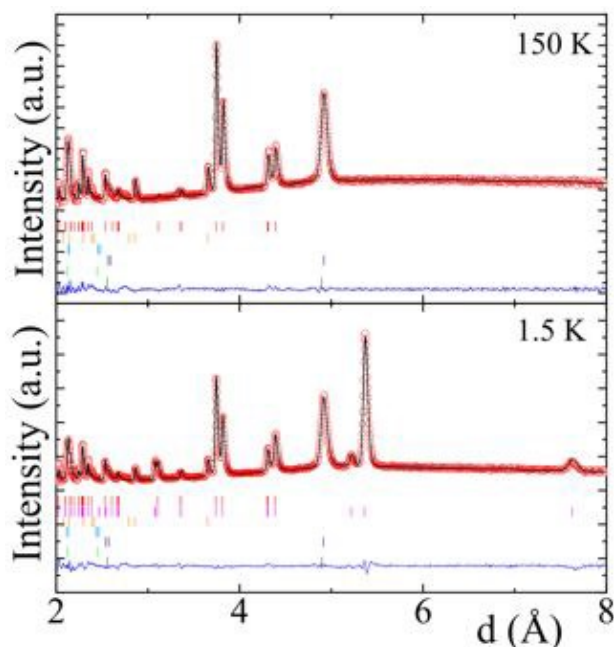
Figure 1. Rietveld fits to 150 and 1.5 K NPD data of \text{Mn}_2\text{NiReO}_6 . Bragg phase markers at 1.5 K from top to bottom are; \text{Mn}_2\text{NiReO}_6 nuclear and magnetic, \text{ReO}_2 , \text{NiO} nuclear and magnetic, and (\text{Ni,Mn})\text{O} nuclear and magnetic.
