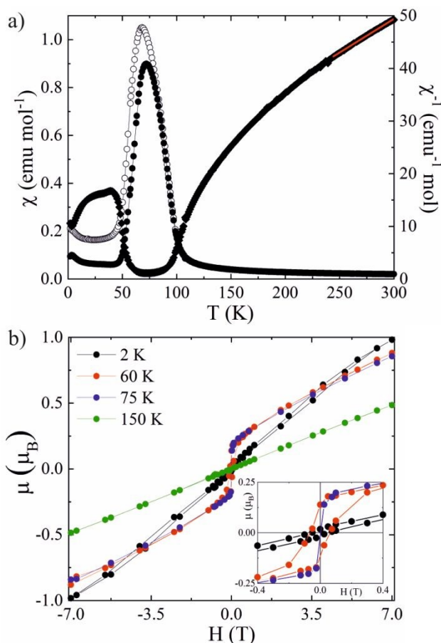
Figure 3. a) Magnetic susceptibility of \text{Mn}_2\text{NiReO}_6 (ZFC/FC = closed/open symbols) and the reciprocal ZFC data with Curie-Weiss fit shown. b) Magnetisation-field hysteresis loops at several temperatures with the low field region of the spin-ordered regime in the inset.
