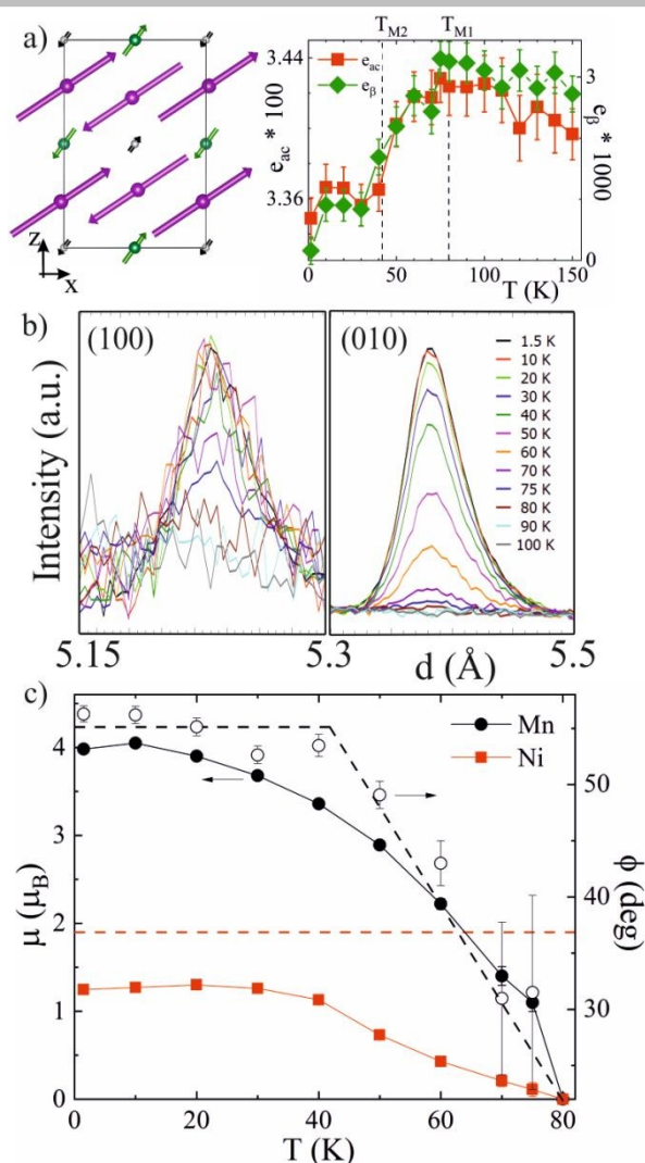
Figure 4. a) Magnetic structure of \text{Mn}_2\text{NiReO}_6 at 1.5 K. The right panel shows the thermal variation strain of the e_{ac} and e_b parameters. b) Plots of (100) and (010) magnetic peaks showing their different thermal evolutions. c) Thermal evolution of the refined magnetic moments and angles \phi (closed and open symbols, respectively) for \text{Mn}^{2+} and \text{Ni}^{2+} site spins. \text{Re}^{6+} moments were constrained to take half the value of those for \text{Ni}^{2+} .
