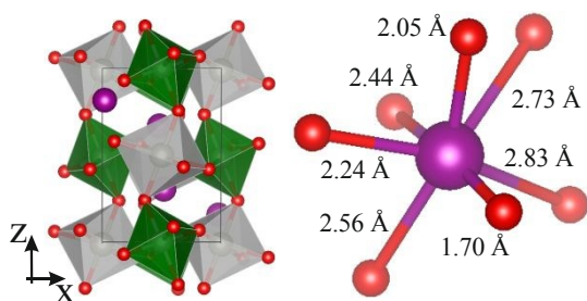
Figure 2. Structure of the double perovskite \text{Mn}_2\text{NiReO}_6 , as refined from 150 K NPD data. Mn is shown as purple spheres and Ni and Re octahedra are green and grey respectively. The coordination of \text{Mn}^{2+} in the A site is depicted on the right.
