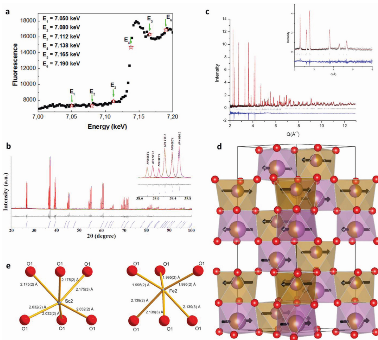
Figure 5. (a) Fluorescence intensity versus energy at the Fe K edge for ScFeO 3 on instrument I11 at DLS. The six selected energy levels ( E_n = 7.050, 7.080, 7.112, 7.138, 7.165, and 7.190 keV for n = 1-6 , respectively) used for diffraction studies near the Fe K absorption edge were marked by arrows (↓) and stars (☆). (b) Simultaneous Rietveld refinement of X-ray diffraction data for ScFeO 3 collected at six selected energy levels near the Fe K absorption edge, giving a partially ordered composition of [\text{Sc}_{0.54(2)}\text{Fe}_{0.46(2)}][\text{Sc}_{0.46(2)}\text{Fe}_{0.54(2)}]\text{O}_3 . The inset ( 38.6-39.8^\circ ) shows the peak evolution and changes in diffraction intensity due to the energy variation of resonant scattering. (c) Rietveld refinement of neutron powder diffraction data (POLARIS 145° bank) for ScFeO 3 ; black crosses represent observed data, the red line the calculated fit, the blue line the difference, upper black tick marks the allowed nuclear Bragg peaks, and the lower ones the allowed magnetic peaks; the inset shows longer d -spacing data from the 35° bank of POLARIS. (d) Polyhedral representation of the final structure viewed along [110]. Brown polyhedra are 54% Fe, 46% Sc, and purple polyhedra are 54% Sc, 46% Fe. Arrows represent the refined magnetic moment orientations. Local coordination environment of (e) the scandium rich site Sc2 and the iron rich site Fe2 viewed perpendicular to the c axis.
