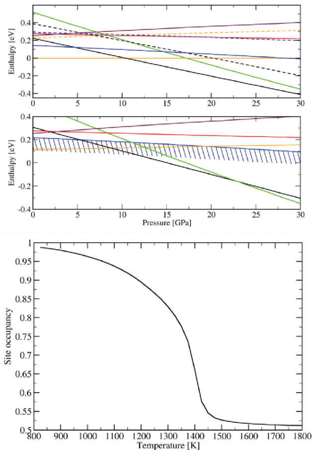
Figure 6. Calculated enthalpies as a function of pressure for \text{ScFeO}_3 polymorphs: polar corundum (blue), perovskite (black), \text{YMnO}_3 (purple), ilmenite (red), and postperovskite (green) relative to the binary oxides (yellow). Upper plot: 0 K results, for FM (solid lines) and AFM (dashed lines) phases. Mid plot: 1773 K results, for the paramagnetic phase, where the blue area represents the contribution of the configurational entropy to the polar corundum, with the lower bound shown representing the maximum possible stabilizing contribution. Both magnetic and configurational terms are essential for the polar corundum to become the stable phase between 0 and 12 GPa. Bottom diagram: temperature dependence of cation order in polar corundum SFO from MC simulations, showing a transition from a mainly ordered to a mainly disordered structure between 1300 and 1450 K.
