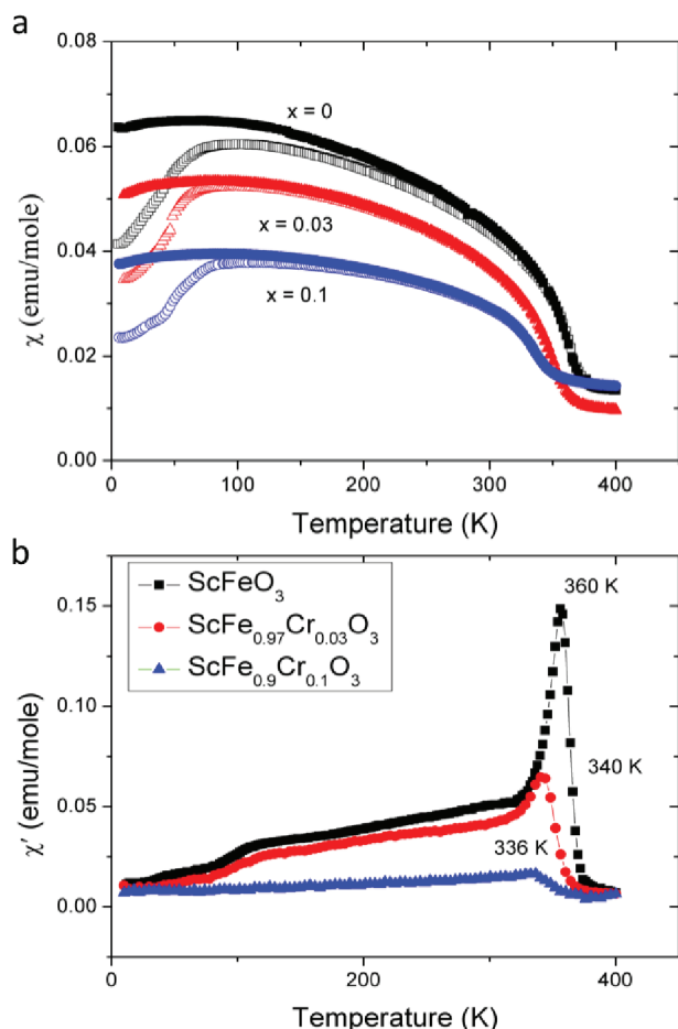
Figure 10. (a) Temperature dependence of the ZFC and FC dc magnetic susceptibility of \text{ScFe}_{1-x}\text{Cr}_x\text{O}_3 ( x = 0, 0.03 , and 0.10 ), measured at 1000 Oe. Open and closed symbols represent ZFC and FC data, respectively. (b) Temperature dependence of the real part of the ac susceptibility of \text{ScFe}_{1-x}\text{Cr}_x\text{O}_3 ( x = 0, 0.03 , and 0.10 ), measured at 5 Oe.
