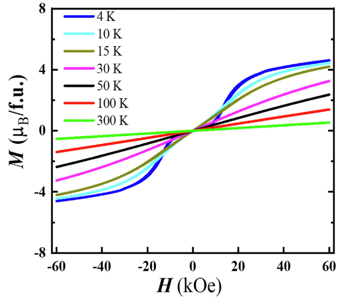
Fig. 3. Magnetization, M , as function of magnetic field, H , for \text{HoCrWO}_6 .
