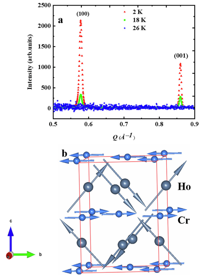
Fig. 7. Magnetic structure determination of \text{HoCrWO}_6 . (a) Comparison of magnetic peaks of \text{HoCrWO}_6 at different temperatures (b) Magnetic structure of \text{HoCrWO}_6 at T = 2 \text{ K} viewed along a -axis. Red lines represent boundary of unit cell. (For interpretation of the references to colour in this figure legend, the reader is referred to the web version of this article.)
