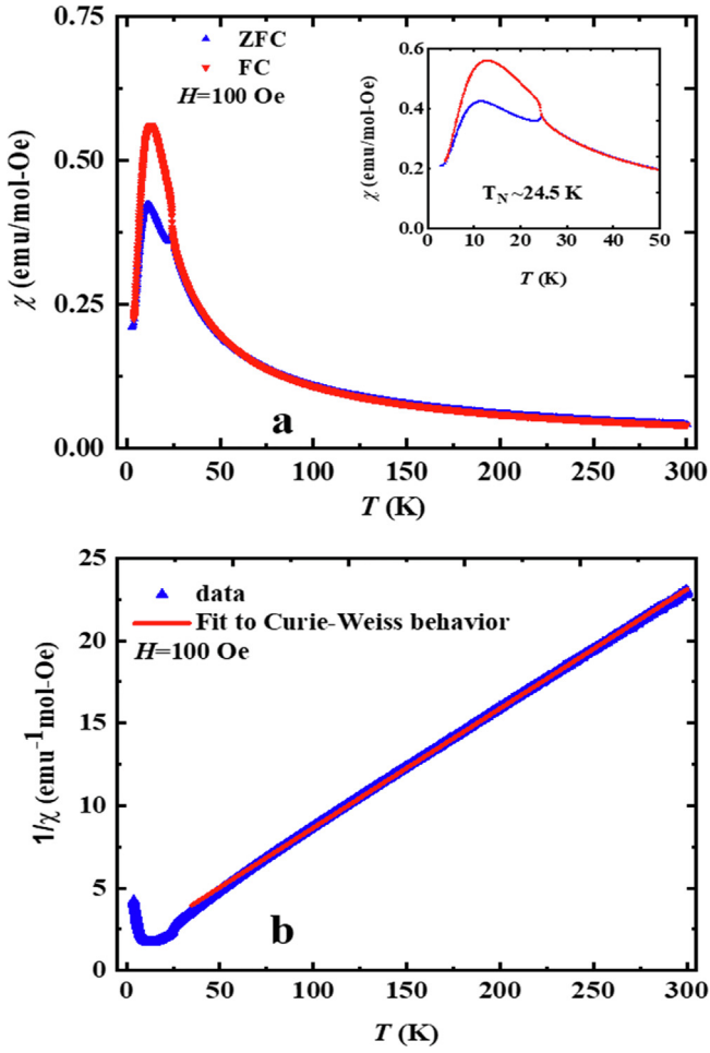
Fig. 2. Magnetic properties of \text{HoCrWO}_6 . (a) The ZFC and FC magnetic susceptibility, \chi , versus temperature, T , measured at H = 100 Oe. Inset: zoomed in \chi versus T curve around the magnetic transition. (b) The inverse susceptibility is plotted against temperature and fitted to \frac{1}{\chi} = \left(\frac{1}{C}\right)T - \left(\frac{\theta}{C}\right) , where C is the Curie-Weiss constant and \theta is the Curie-Weiss temperature. The red line is the fit to data in the temperature range 300 K to 35 K. (For interpretation of the references to colour in this figure legend, the reader is referred to the web version of this article.)
