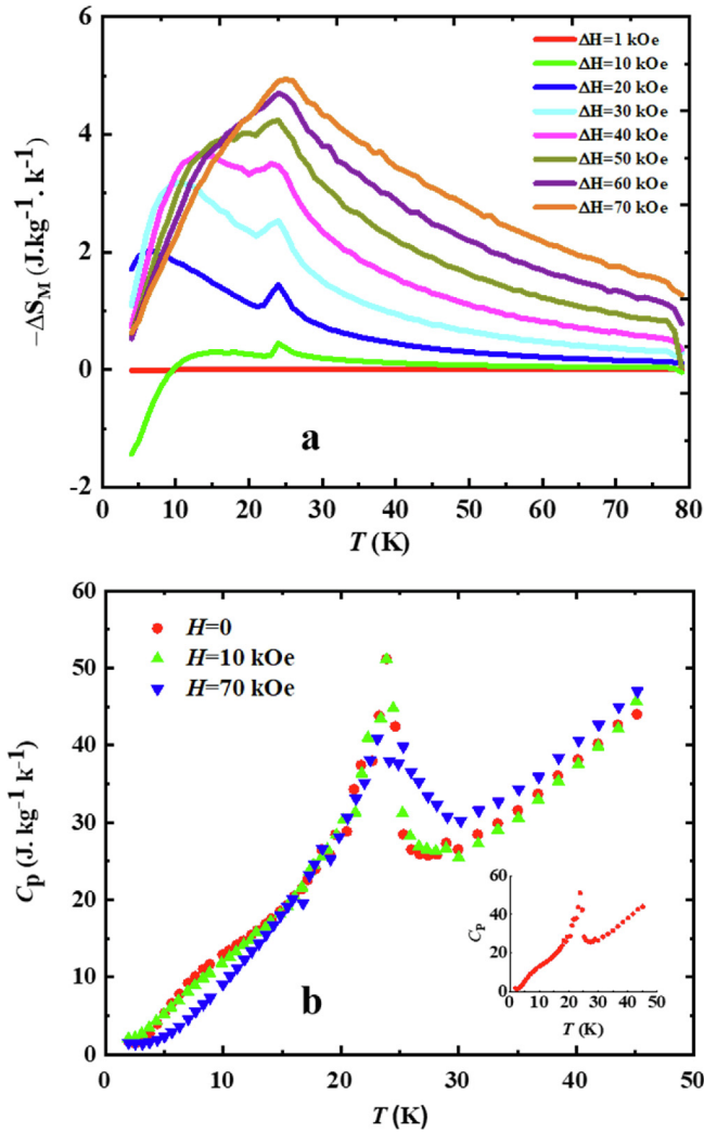
Fig. 5. (a) Change in the magnetic entropy as function of temperature for different fields. (b) Heat capacity, C_p , vs T . Inset shows specific heat measured at zero field.
