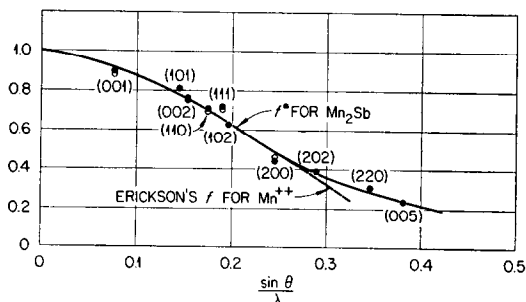
FIG. 8. Magnetic amplitude form factor for manganese atoms in \text{Mn}_2\text{Sb} . The solid points represent data on specimens cut from Crystal H , and open circles represent data on specimens cut from Crystal M .
