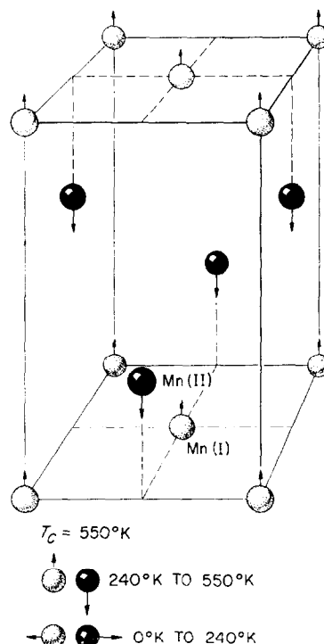
FIG. 1. Magnetic structure proposed for \text{Mn}_2\text{Sb} by GUILLAUD from magnetic measurements. Suggested values of atomic magnetic moments were +3 \mu_B for Mn(I) and -5 \mu_B for Mn(II).
