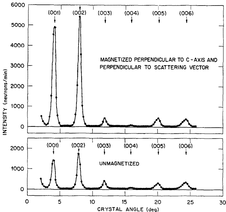
FIG. 4. Neutron diffraction patterns of the (00l) single-crystal reflections from \text{Mn}_3\text{Sb} .
