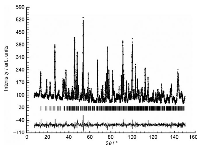
Figure 2. Observed (circles), calculated (solid line), and difference (at the bottom) neutron diffraction (D1A, ILL) profiles for \text{KCo}_4(\text{PO}_4)_3 at room temperature. Vertical marks correspond to the position of the allowed reflections for the crystallographic structure.
