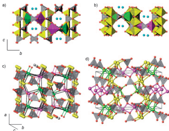
Figure 3. Crystal structure of \text{KM}_4(\text{PO}_4)_3 . Projection along the [100] direction for \text{M}=\text{Mn} (a) and \text{M}=\text{Co} (b). Projection along the [001] direction for \text{M}=\text{Mn} (c) and \text{M}=\text{Co} (d). Colour codes: M1 pink, M2 green, and M3 yellow; \text{PO}_4 groups dark-grey tetrahedra; K blue.
