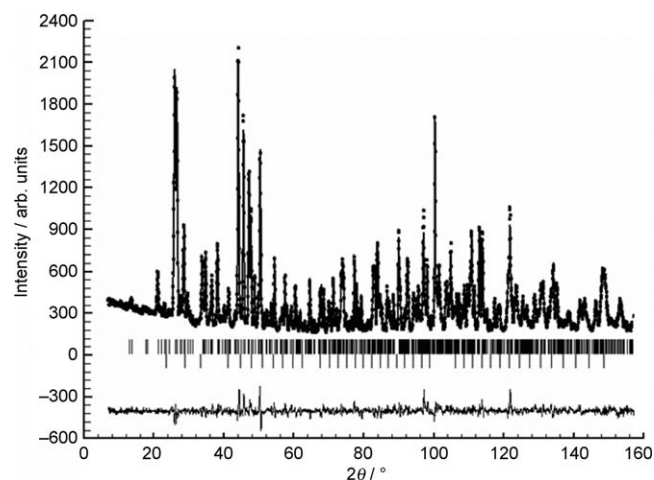
Figure 1. Observed (circles), calculated (solid line), and difference (at the bottom) neutron diffraction (D1A, ILL) profiles for \text{KMn}_4(\text{PO}_4)_3 at room temperature. Vertical marks correspond to the position of the allowed reflections for the crystallographic structure. The second series of tick marks corresponds to the Bragg reflections of the \text{Mn}_2\text{O}_3 impurity phase.
