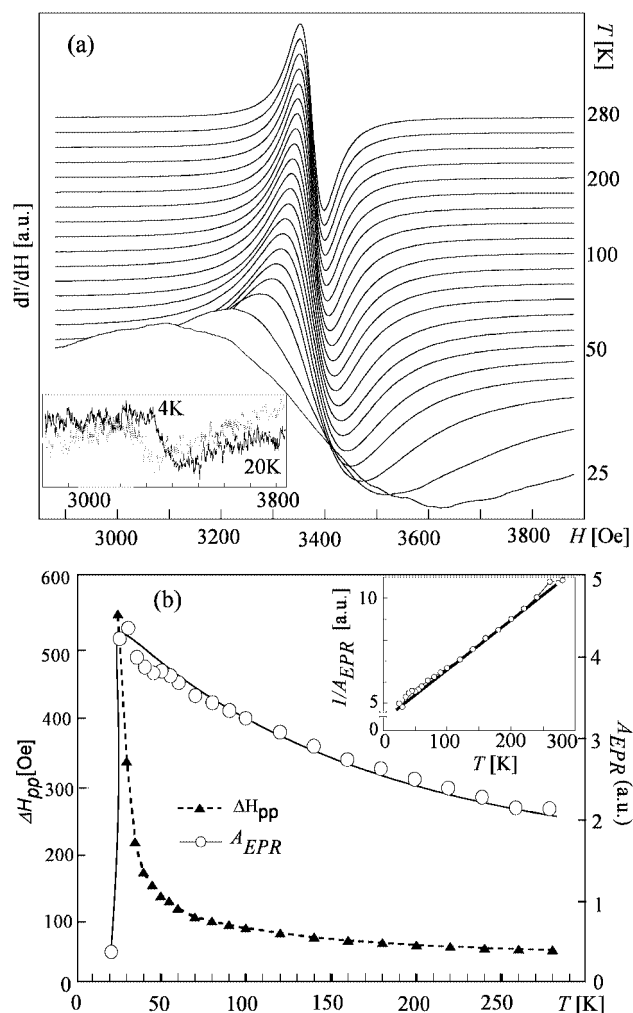
Figure 2. (a) Normalized EPR spectra between 280 and 25 K. The inset shows the weak EPR spectra observed at 4 and 20 K. (b) Thermal evolution of the signal area ( A_{\text{EPR}} ) and the peak-to-peak linewidth ( \Delta H_{\text{pp}} ).
