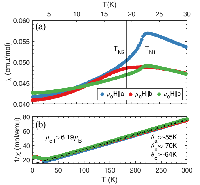
FIG. 3. (a) displays the temperature dependence of the susceptibility \chi for all crystallographic directions around the phase transitions T_{N1} and T_{N2} . The susceptibility was measured after zero-field cooling, while heating and applying a constant field of \mu_0 H = 0.1 T to the sample. Curie-Weiss fits for 1/\chi are shown by dashed black lines in (b) together with the resulting Weiss temperatures \theta and the averaged effective moment \mu_{\text{eff}} .
