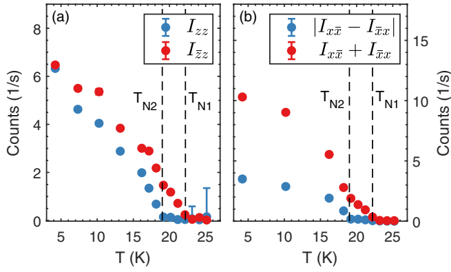
FIG. 7. The displayed intensities in (a) correspond to the recorded NSF and SF channels I_{zz} and I_{\bar{z}z} with \mathbf{P}||z and \mathbf{Q} = (-1.09 \ 0 \ 0.30) . In (b) the sum and the difference of both SF channels with \mathbf{P}||x are plotted.
