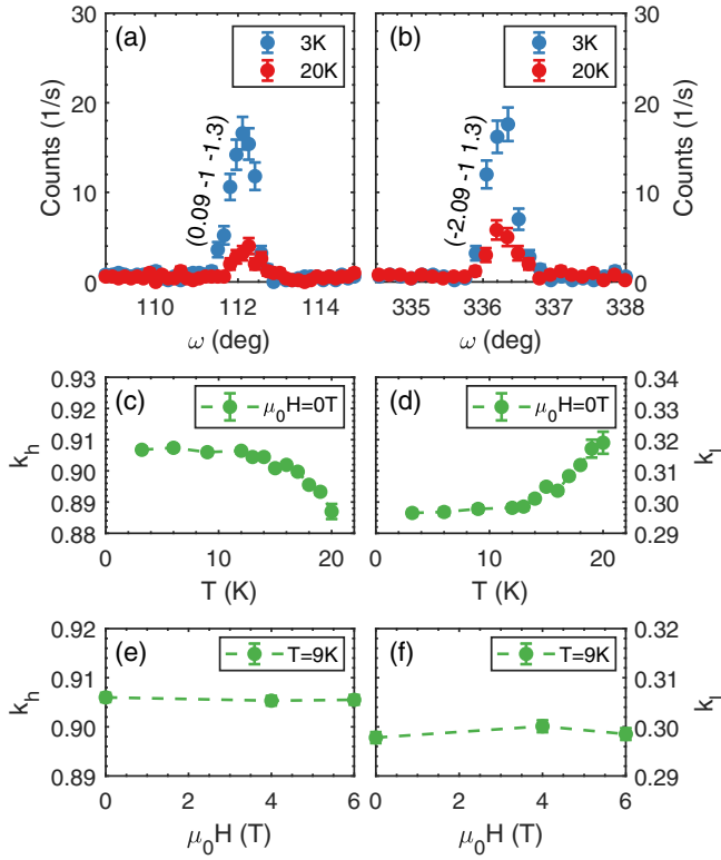
FIG. 4. (a) and (b) display rocking scans over the magnetic reflections \mathbf{Q} = (0.09 -1 -1.30) and \mathbf{Q} = (-2.09 -1 1.30) for T = 3 K and T = 20 K, respectively. The temperature and magnetic-field dependences of the incommensurate propagation vector \mathbf{k}_{\text{inc}} = (k_h, 0, k_l) are shown in (c)–(f). All respective values have been obtained by fitting the \mathbf{Q} -space mappings in the h - l plane with a two-dimensional Gaussian function. The magnetic field was applied along the b direction.
