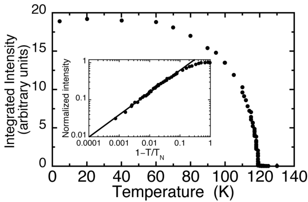
Figure 8. Integrated intensity of the (0 1 0) Bragg peak as a function of temperature. The Néel temperature was established to be 119.1 \pm 0.1 K. The insert shows the normalized data plotted against reduced temperature with a fit to a power law. The fitted exponent was found to be 2\beta = 0.60 \pm 0.01 . The estimated standard deviations are within the sizes of the data points.
