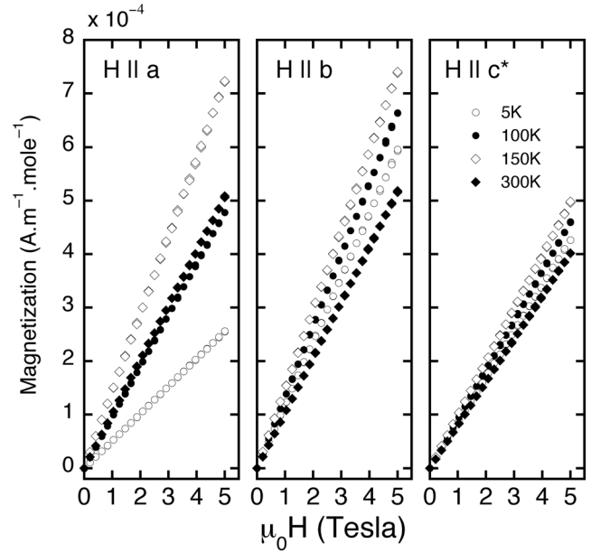
Figure 2. Magnetization as a function of applied field along different crystallographic directions. The measurements were performed using the MPMS magnetometer. The estimated standard deviations are within the sizes of the data points.
