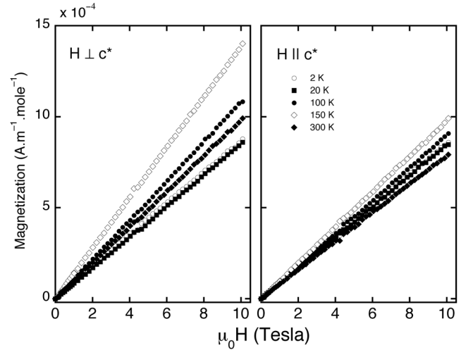
Figure 3. Magnetization as a function of applied field for the field parallel and perpendicular to the c* axis. The measurements were performed using the BS2 magnetometer. The estimated standard deviations are within the sizes of the data points.
