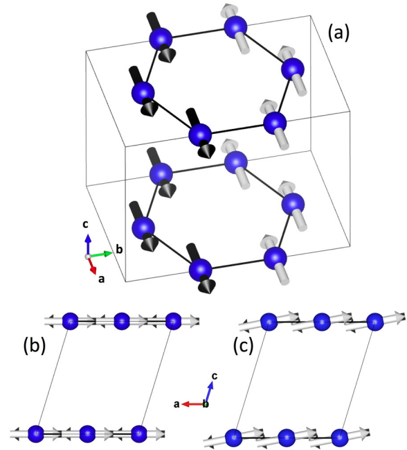
Figure 7. Magnetic structure for \text{CoPS}_3 . (a) Isometric view of the unit cell. (b) View along the b -axis for the previously-published structure [7], showing the moments lying along the a axis. (c) View along the b axis for the refined structure in the present work, showing a small out-of-plane component to the moments.
