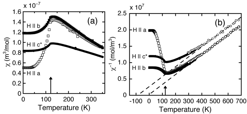
Figure 1. The (a) susceptibility; and (b) inverse susceptibility for a single crystal of CoPS 3 . The field was applied along different directions for the measurements, which are marked in the figure. Data between 2 and 350 K were measured using a MPMS SQUID magnetometer with an applied field of 0.1 Tesla, while the BS1 magnetometer was used to collect data between 300 and 680 K. Fits of a straight line to the high-temperature inverse susceptibility data for H parallel and perpendicular to \mathbf{c}^* are shown. The arrows mark the expected Néel temperature of 122 K. The estimated standard deviations are within the sizes of the data points.
