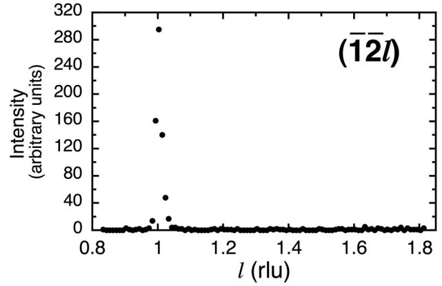
Figure 5. Neutron diffraction measurement from D10 along (\bar{1}2l) of CoPS 3 at 4 K.
