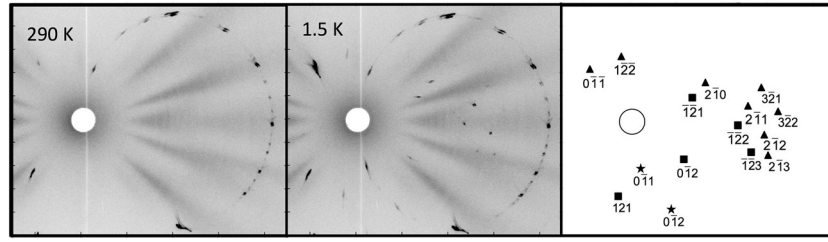
Figure 4. Neutron Laue diffraction patterns of CoPS 3 at 290 K (left panel) and 1.5 K (middle panel). The new Laue spots at 1.5 K are due to the onset of long-ranged antiferromagnetic order. The Miller indices for the new spots are shown in the right panel. The different symbols (triangle, square, star) in the right panel represent the crystallographic domains used to index the spots and the circle, included as a positioning aid, indicates the hole in the image plate for the passage of the neutron beam.
