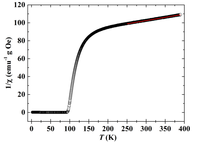
FIG. 5. Temperature dependence of inverse susceptibility of \text{LiFeCr}_4\text{O}_8 at 0.1 kOe. The linear fitting of the inverse susceptibility data in the temperature range of 250–390 K is shown in red.
