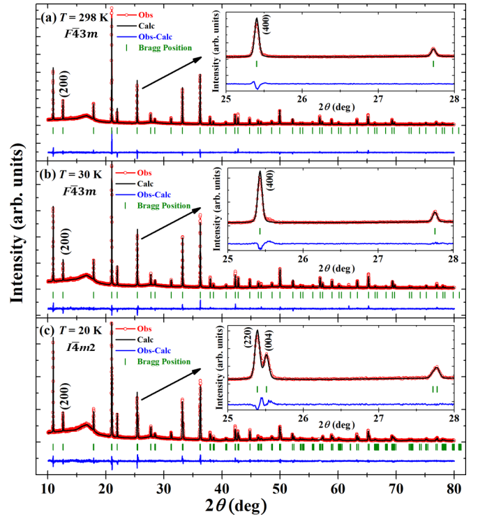
FIG. 1. Rietveld refinements on the synchrotron x-ray diffraction data of \text{LiFeCr}_4\text{O}_8 collected at (a) 298 K, (b) 30 K, and (c) 20 K with \lambda = 0.91 Å. Insets of (a)–(c) show the lowering of symmetry from (a),(b) F\bar{4}3m to (c) I\bar{4}m2 upon cooling below the magnetostructural transition ( T_{MS} \sim 23 K).
