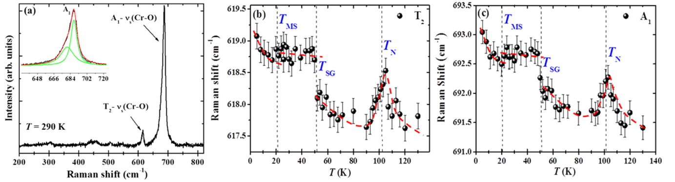
FIG. 10. (a) Raman spectra of \text{LiFeCr}_4\text{O}_8 at 290 K. The inset shows the deconvolution of the Cr-O stretching mode ( A_1 ); (b),(c) Temperature dependence of the T_2 (left panel) and A_1 (right panel) modes. The dashed lines correspond to the transition temperatures and the red lines are a guide to the eyes.
