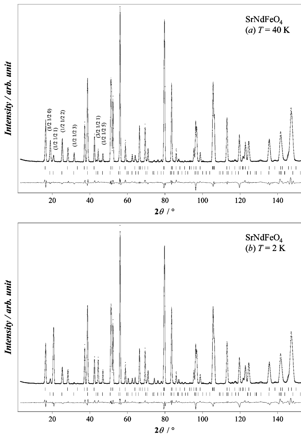
Figure 8. Powder neutron diffraction profiles for \text{SrNdFeO}_4 at 40 (a) and 2 K (b). The calculated and observed diffraction profiles are shown by the top full curve and the cross markers, respectively. The nuclear reflection positions are shown as upper vertical markers and magnetic ones are shown as lower ones. The lower trace is a plot of the difference between calculated and observed intensities.
