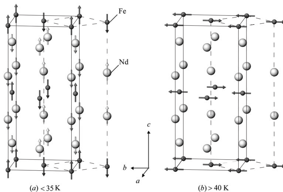
Figure 10. Magnetic structure models of \text{SrNdFeO}_4 below 35 K (a) and above 40 K (b). Diamagnetic ions are omitted. Arrows show the direction of the magnetic moments.
