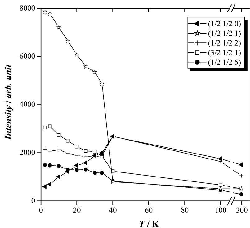
Figure 9. Temperature dependence of the integrated intensities of some magnetic Bragg reflections for \text{SrNdFeO}_4 .
